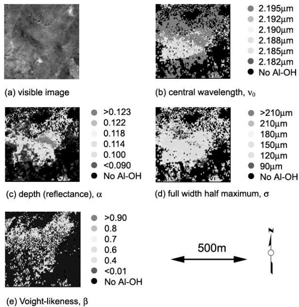
Fig. 2. Maps of Al-OH band parameters. (a) visible image (b) central wavelength, v_0 (c) depth of absorption band, \alpha (d) full width half maximum, \sigma (e) Voight-likeness parameter, \beta . Values given are the bottom of each range defined by different colors. Note – a color version of this image is available on IEEE Explore in the ‘Multimedia’ link next to the PDF ‘link’ for this paper.
