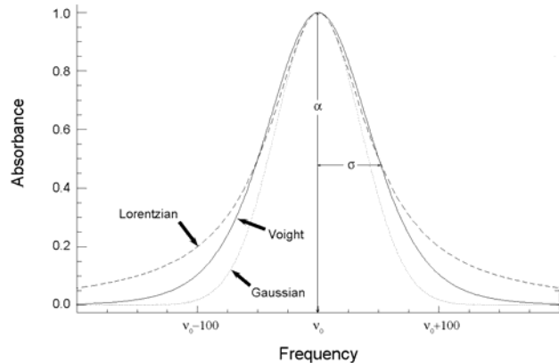
Fig. 1. Comparison of Gaussian, Lorentzian and Voight functions describing an ideal, symmetrical absorption band. For each function, \alpha=1 , \sigma=100 . The Voight function has been generated as described in the text, with \beta=0.5 .
